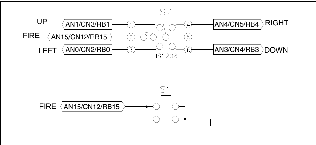
FIGURE 2-11: JOYSTICK AND FIRE BUTTON CONNECTION SCHEMATIC
