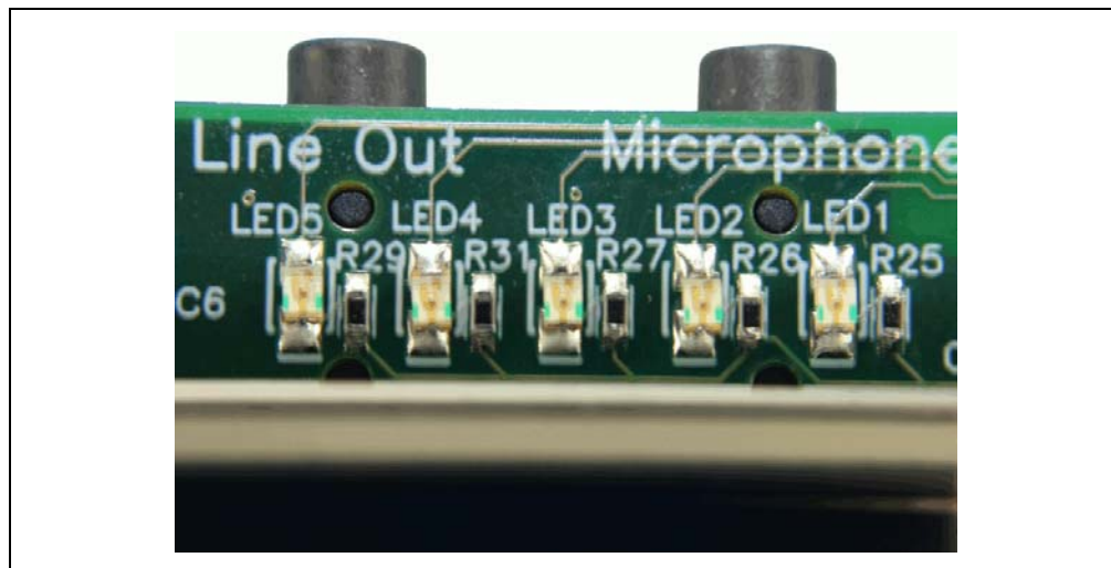
FIGURE 2-12: LEDS
