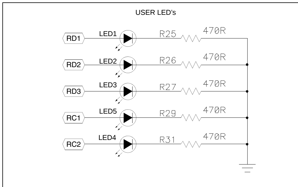
FIGURE 2-13: LED CONNECTION SCHEMATIC
