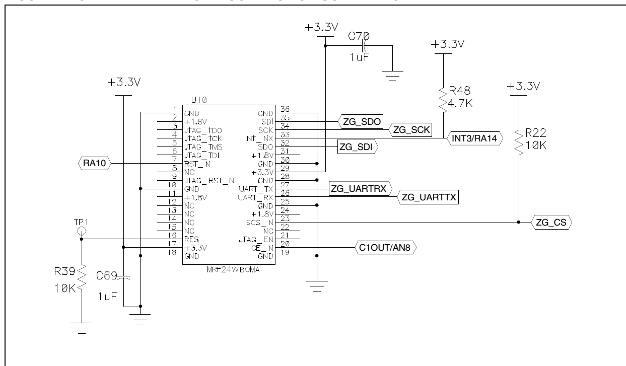
FIGURE 2-25: MRF24WB0MA CONNECTION SCHEMATIC
