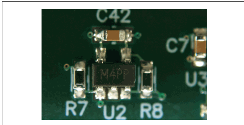
FIGURE 2-16: 24LC08 EEPROM
