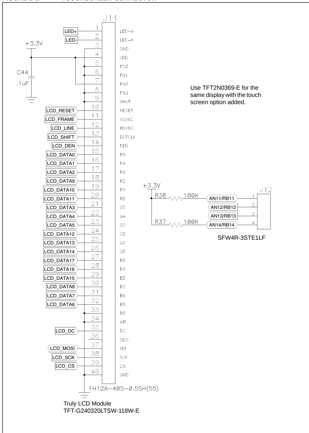
FIGURE 2-6: TOUCHSCREEN CONNECTOR
