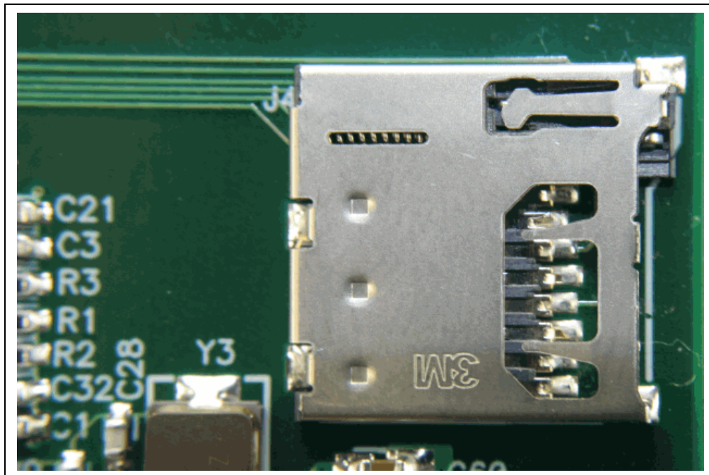
FIGURE 2-7: microSD CARD SLOT
