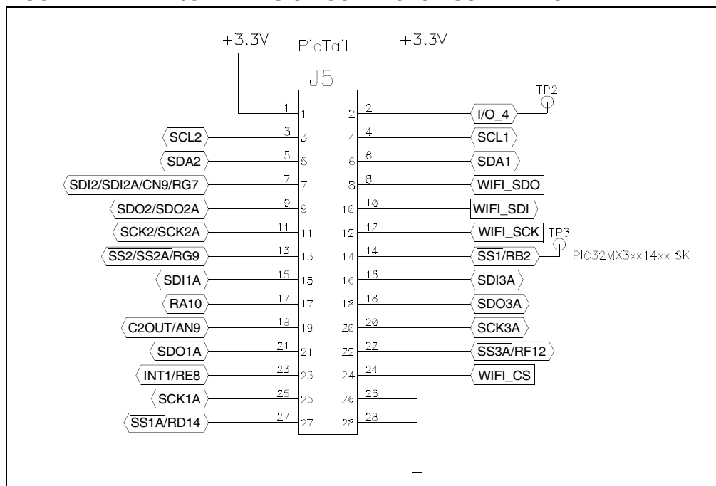
FIGURE 2-27: I/O EXPANSION CONNECTOR SCHEMATIC
